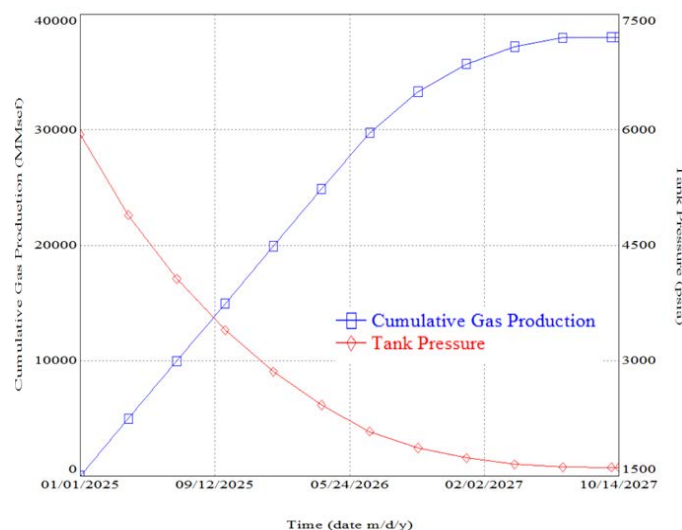
Figure 6: Production forecast using 5.5-in tubing
